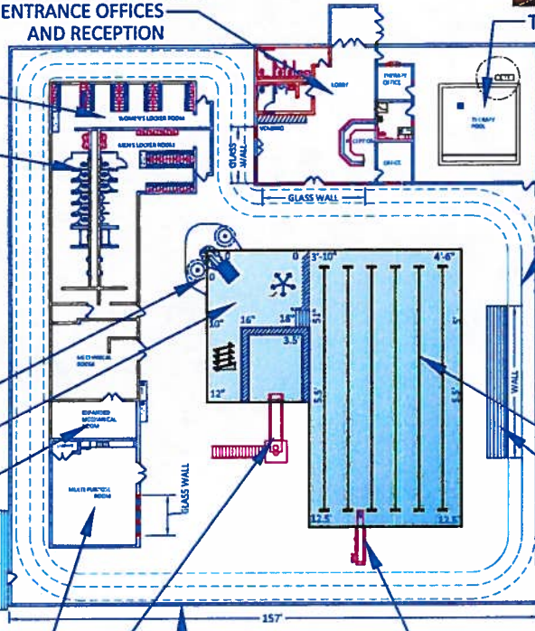
NATATORIUM TENSION MEMBRANE STRUCTURE
